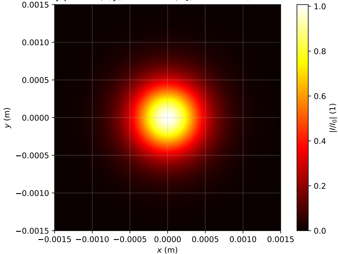
Intensity profile I(x, y, z = 1.751m)/I_0 , Pin=0.6Pcr, artificial time
